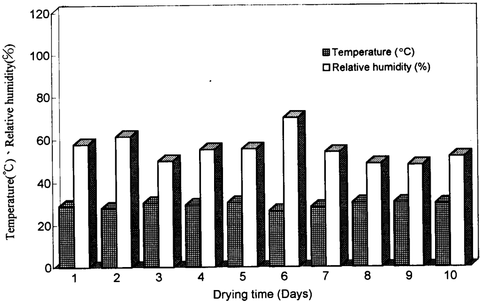
圖 2. 以除濕乾燥法製造柿餅期間之溫度、相對濕度及電力消耗之變化 Fig. 2. Changes in temperature and relative humidity during dehumidification drying of persimmons.
